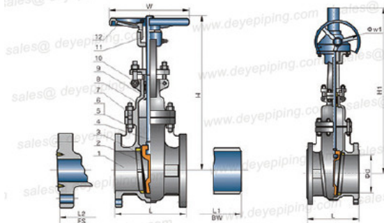
美标150Lb铸钢闸阀 Class 150 Cast Steel Gate Valve
