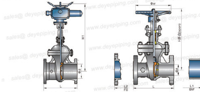
美标300Lb铸钢闸阀 Class 300 Cast Steel Gate Valve
